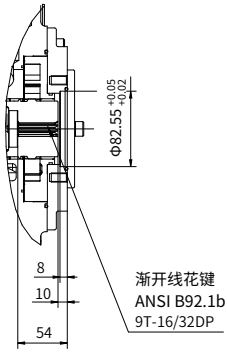
“A1”型通轴驱动
