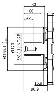
“E3” 型花键轴
